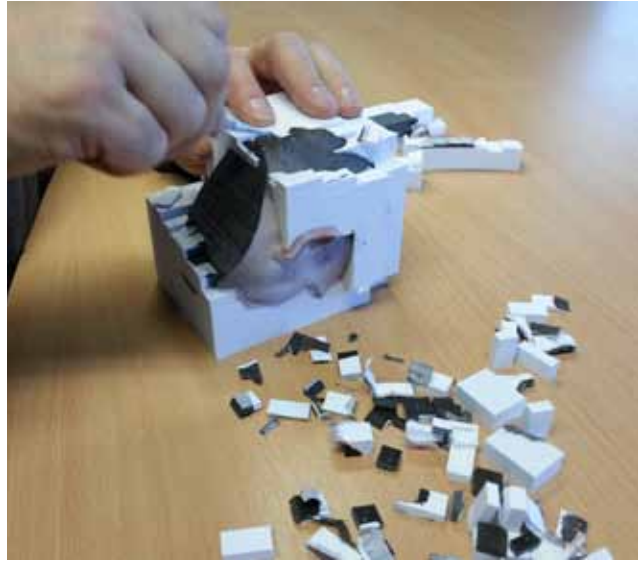
Fig. 4 Quickly and easily peel the supporting paper away from the part. This can be accomplished with your hands and ordinary tweezers; no need for chemicals. The head model emerges.
