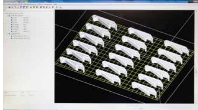
Fig. 1 Mcor's SliceIT software reads the digital data and slices the computer model into printable layers equivalent in thickness to the paper. Compatible file formats are STL, OBJ and VRML.
